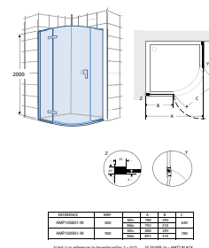
Metropolis-N MRF
